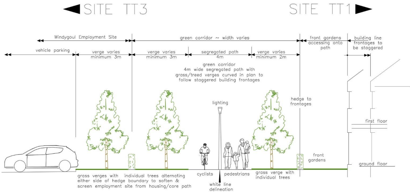
TYPICAL SECTION THROUGH CORE PATH 345 EAST (NORTH TO SOUTH) ~ NOT TO SCALE ~
