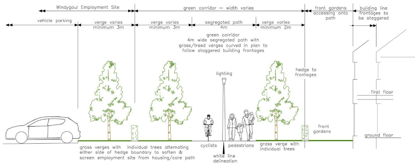
TYPICAL SECTION THROUGH CORE PATH 345 EAST (NORTH TO SOUTH)
